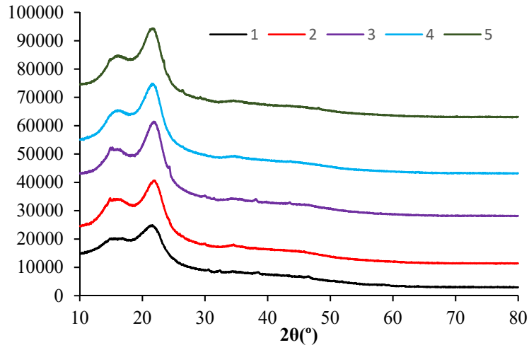
Figure 5 X-ray diffraction patterns for different powder samples (1) Artichoke, (2) Spruce, (3) Savle, (4) Piank and (5) Myscanyhus
