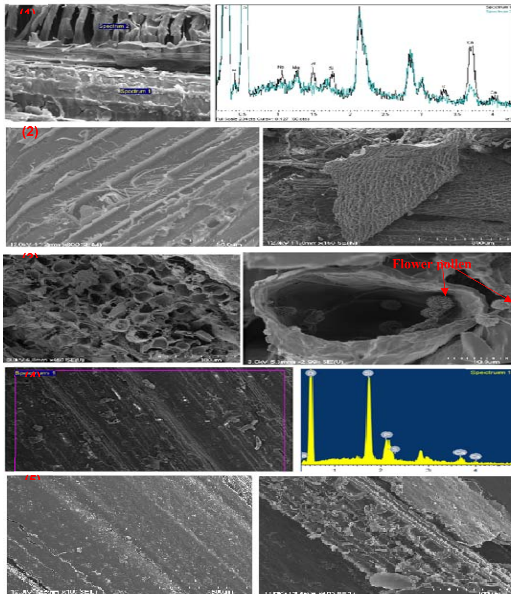
Figure 4 SEM image and EDS of 1) Artichoke waste, 2) spruce waste sample, 3) Savle waste sample, 4) Piangk waste sample, 5) Myscanyhus waste sample.
