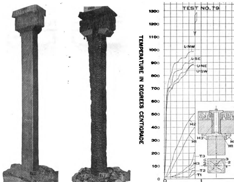
Figure 6. Early Standard fire tests were conducted on timber columns in the early 20 th Century. It was difficult to control these tests due to the heat given off from the timber. Excerpted are the results of the first Standard fire test on un-encapsulated timber (Ingberg 1921).
