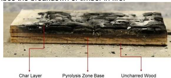
Figure 1. When wood is heated, a material degradation occurs with the creation of a carbon region called char, a weakened (strength) pyrolysis zone, and finally these zones protect an uncharred region.
