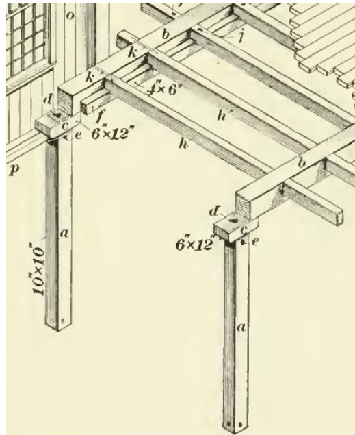
Figure 2. Solid timber was prevalent for a 19 th century industry structure design called slow-burning construction (see Scanton 1899). The timber would be made sufficiently large so that business continuity was ensured if fire damage occurred. The timber would have a hollowed center, which would aid in connection and prevent moisture accumulation that would enable rot.
