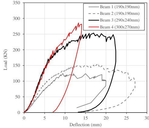
Figure 7. Load and Deflection Behavior of four Heritage Beams (loading and unloading shown).
