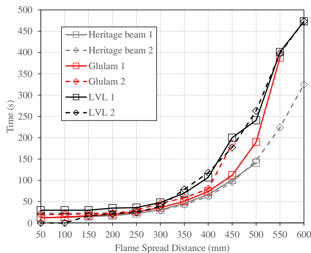
Figure 9. Flame Spread Observations.
