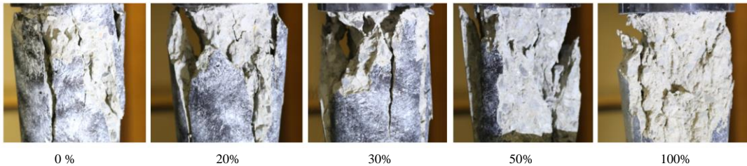
Figure 8: Failure planes with various recycled cement substitution
