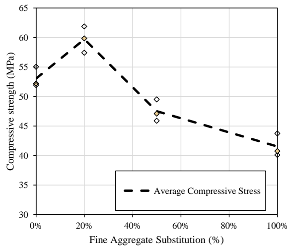
Figure 4: Cylinder compressive strength with fine aggregate substitution
