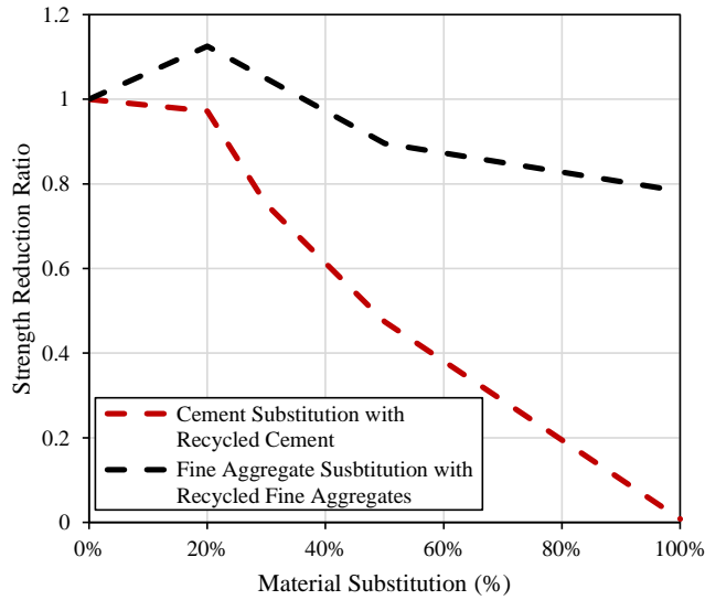
Figure 6: Proposed strength reduction factors
