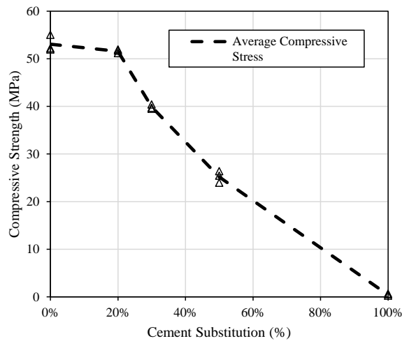
Figure 5: Cylinder compressive strength with recycled cement substitution
