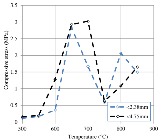
Figure 2: Peak load at increasing temperature for two sieve sizes of RCC
