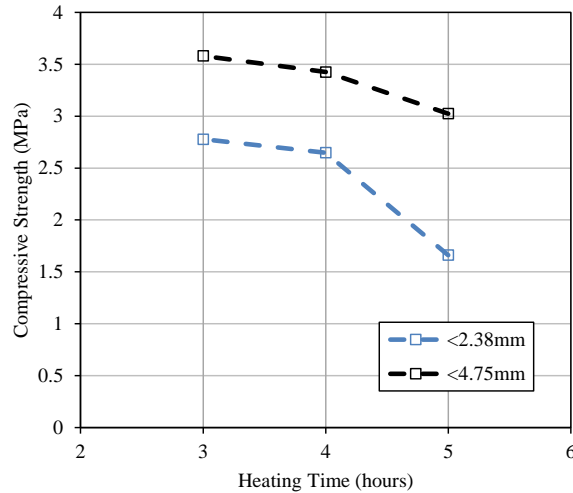
Figure 3: Peak compressive stress with increasing heating time for two sieve sizes of RCC for 650°C
